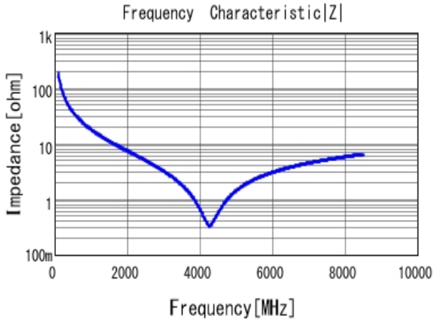
■ GRM0225C1H8R3DA03 |Z| DC0V, 25degC
