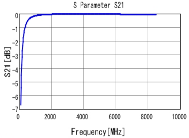
■ GRM0225C1H8R3DA03 S21 DCOV, 25degC
