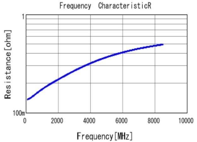
■ GRM0225C1H8R3DA03 R DC0V, 25degC
