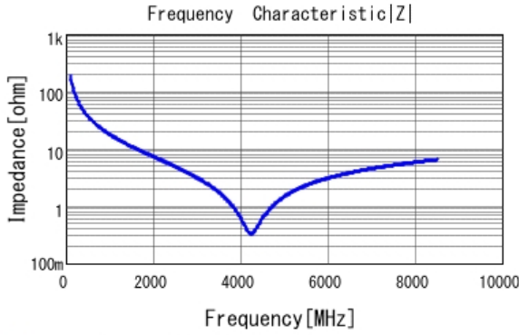
■ GRM0225C1H8R4CA03 |Z| DCOV, 25degC
