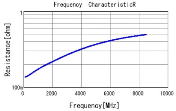
■ GRM0225C1H8R4CA03 R DCOV, 25degC
