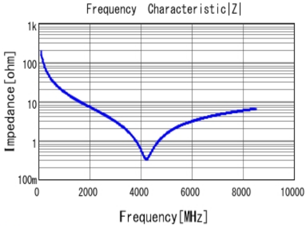
■ GRM0225C1H8R6WA03 |Z| DCOV, 25degC
