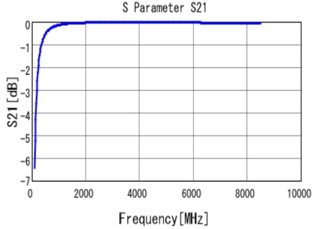
■ GRM0225C1H8R6WA03 S21 DCOV, 25degC
