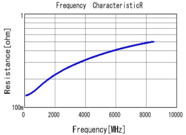
■ GRM0225C1H8R7CA03 R DC0V, 25degC
