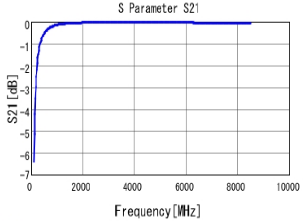
■ GRM0225C1H8R7CA03 S21 DCOV, 25degC
