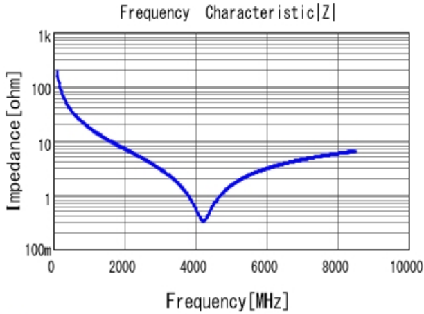
■ GRM0225C1H8R7CA03 |Z| DC0V, 25degC
