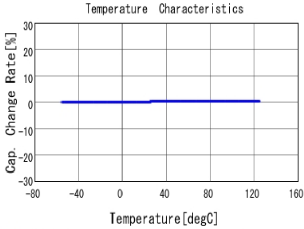
■ GRM0225C1H8R7CA03 C-Temp. capchange, DCOV, AC1Vrms
