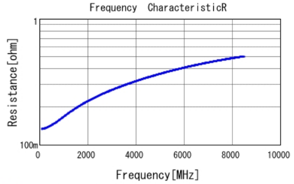
■ GRM0225C1H8R8DA03 R DCOV, 25degC
