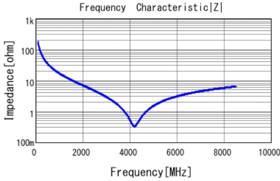
■ GRM0225C1H8R8DA03 |Z| DCOV, 25degC
