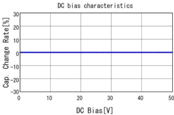
■ GRM0225C1H9R2CA03 C-DC bias capchange, 25.0degC, AC1V
