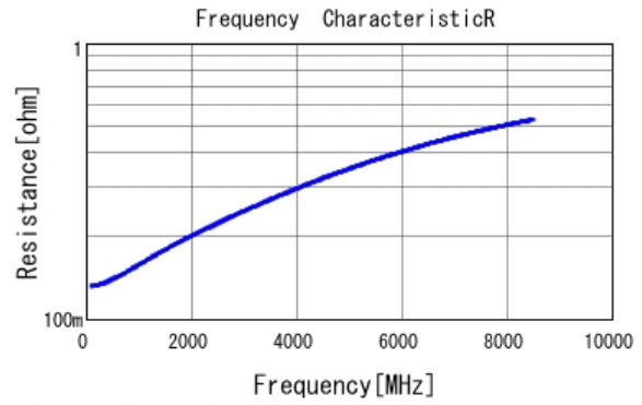
■ GRM0225C1H9R2CA03 R DCOV, 25degC
