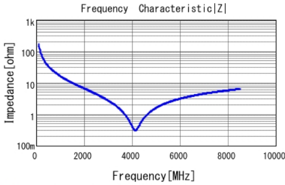
■ GRM0225C1H9R2CA03 |Z| DCOV, 25degC
