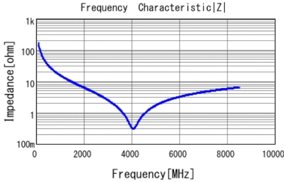
■ GRM0225C1H9R5BA03 |Z| DCOV, 25degC
