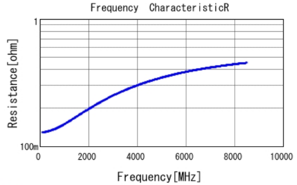
■ GRM0225C1H9R5BA03 R DCOV, 25degC
