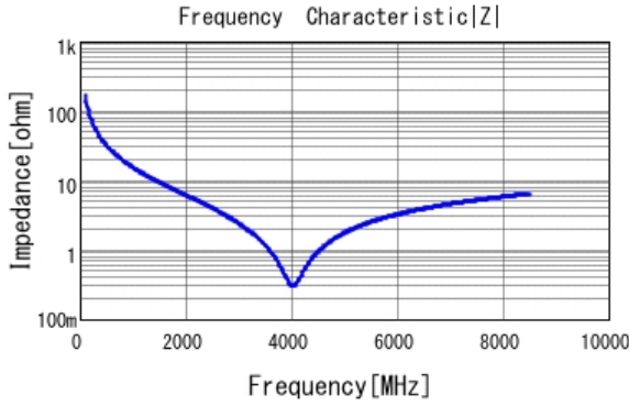
■ GRM0225C1H9R7BA03 |Z| DCOV, 25degC
