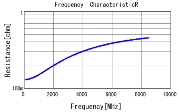
■ GRM0225C1H9R7BA03 R DCOV, 25degC
