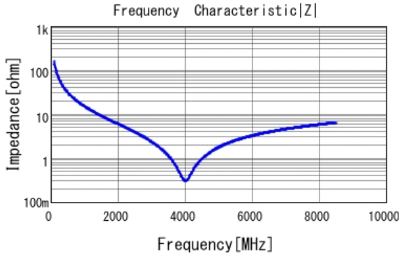
■ GRM0225C1H9R8CA03 |Z| DCOV, 25degC
