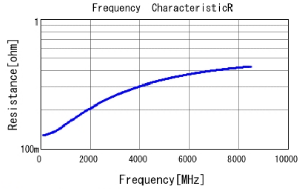
■ GRM0225C1H9R8CA03 R DCOV, 25degC
