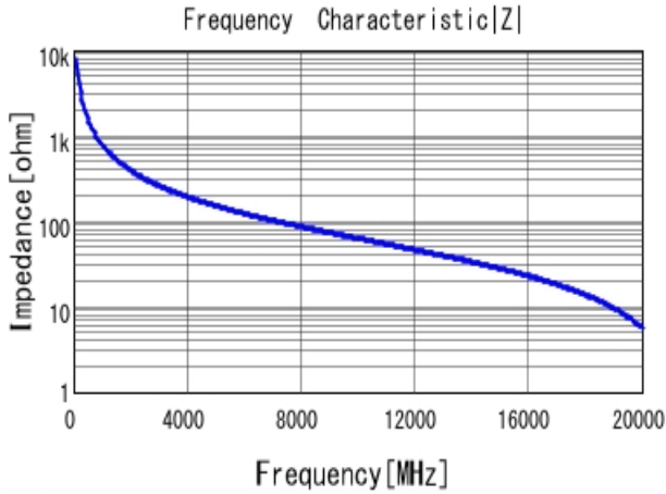
■ GRM0225C1HR20BA03 |Z| DC0V, 25degC
