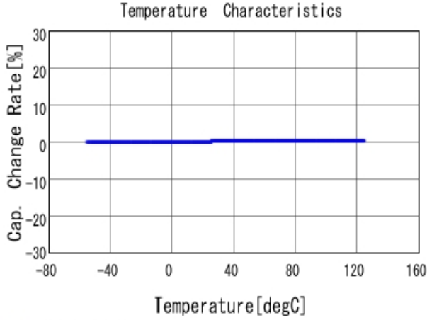
■ GRM0225C1HR20BA03 C-Temp. capchange, DCOV, AC1Vrms
