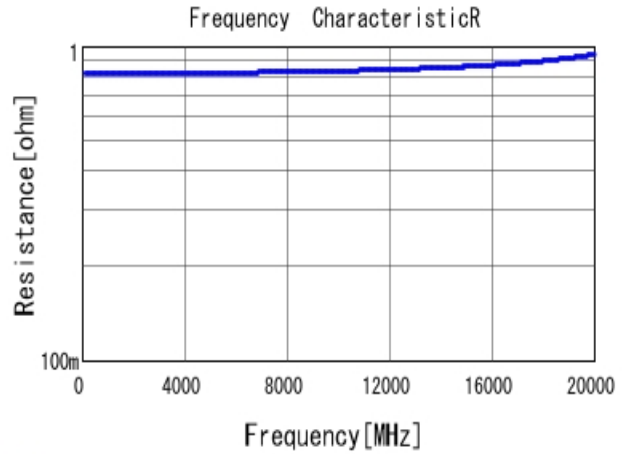
■ GRM0225C1HR20BA03 R DC0V, 25degC
