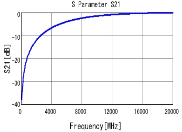
■ GRM0225C1HR20BA03 S21 DCOV, 25degC
