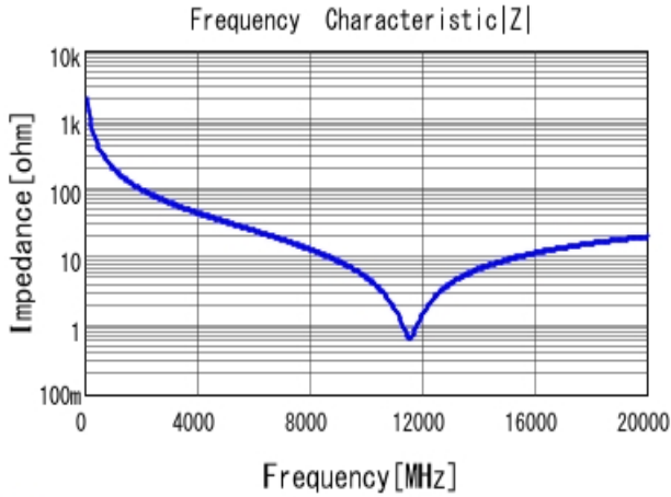
■ GRM0225C1HR80BA03 |Z| DC0V, 25degC
