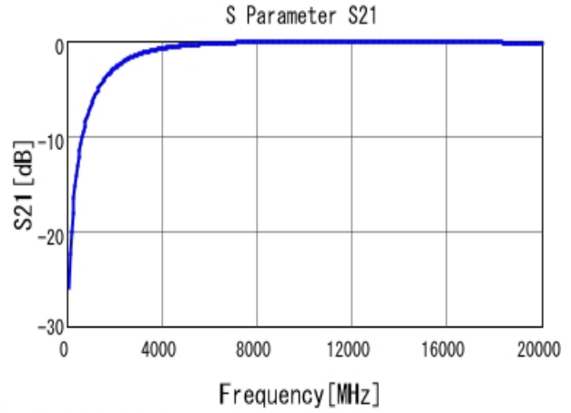
■ GRM0225C1HR80BA03 S21 DCOV, 25degC
