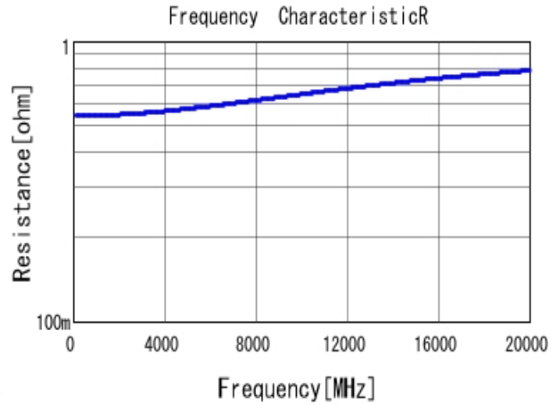
■ GRM0225C1HR80BA03 R DC0V, 25degC
