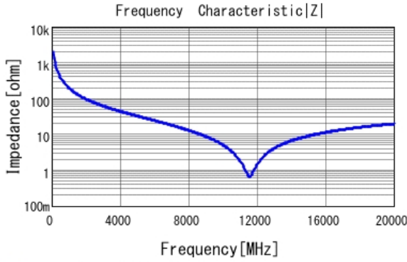
■ GRM0225C1HR80WA03 |Z| DCOV, 25degC
