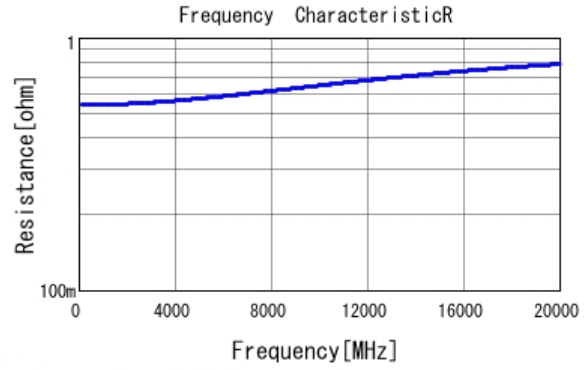
■ GRM0225C1HR80WA03 R DCOV, 25degC
