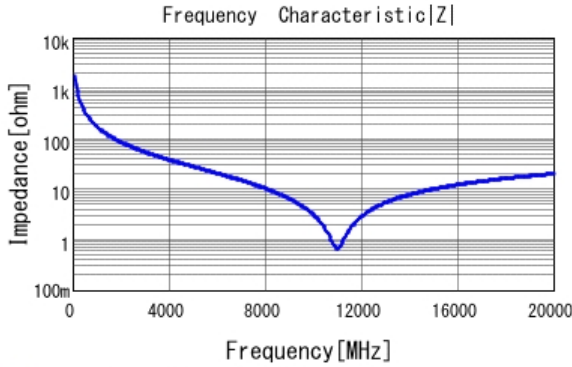
■ GRM0225C1HR90BA03 |Z| DCOV, 25degC
