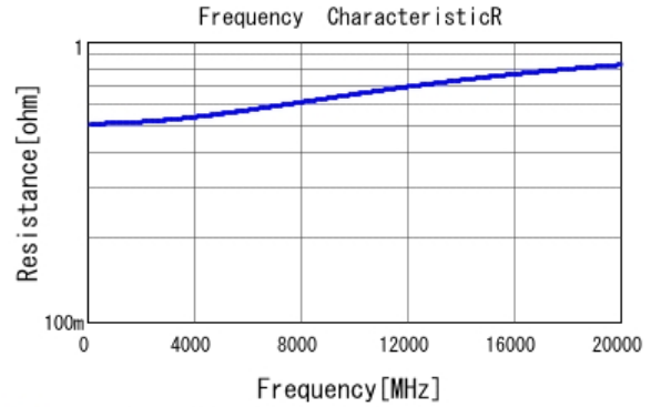
■ GRM0225C1HR90BA03 R DCOV, 25degC
