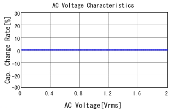
■ GRM0225C1HR90BA03 C-AC Voltage capchange, DCOV, 25.0d
