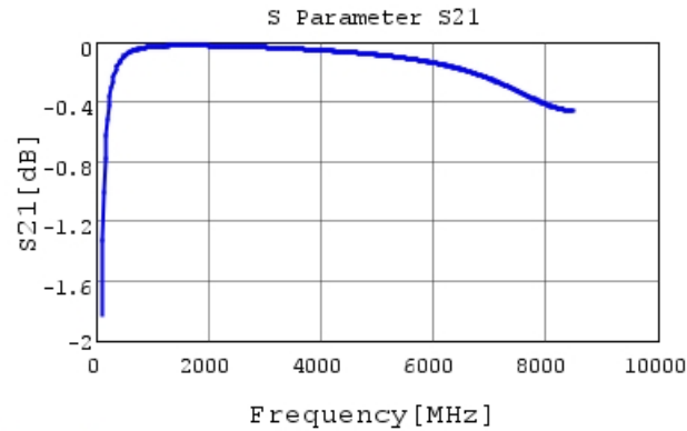
GRM0332C2A220GA01 S21 DCOV, 20degC
