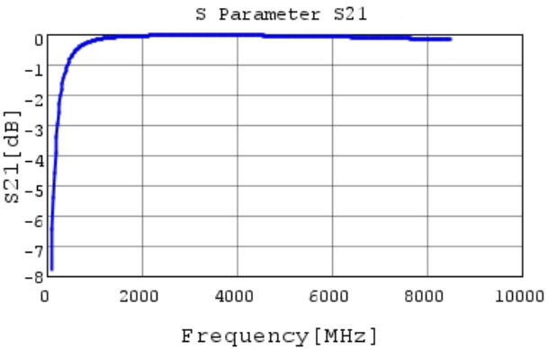
GRM0332C2A7R1DA01 S21 DCOV, 20degC
