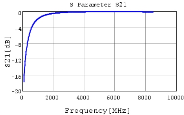
GRM0335C1H2R1BA01 S21 DCOV, 25degC
