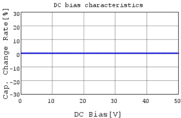
GRM0335C1H6R5CA01 C-DC bias capchange, 25.0C
