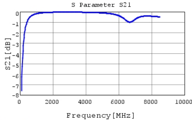
GRM1552C1H7R3WA01 S21 DCOV, 20degC
