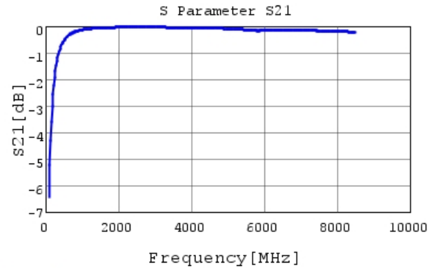
GRM1552C1H8R6WA01 S21 DCOV, 20degC
