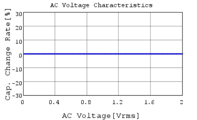
GRM1552C2A6R3CA01 C-AC Voltage capchange, Dc
