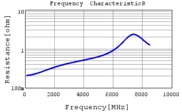
GRM1552C2A6R3CA01 R DCOV, 20degC
