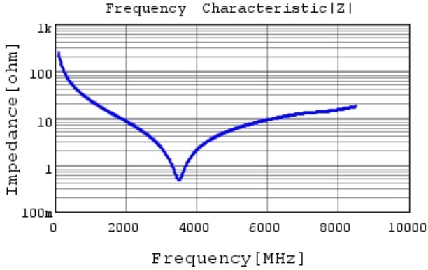
GRM1552C2A6R3CA01 |Z| DCOV, 20degC
