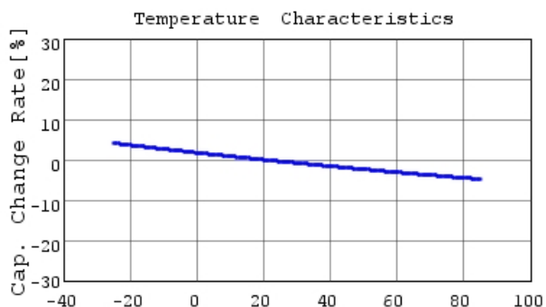
GRM1553U1A122JA01 C-Temp. capchange, DCOV, 1
