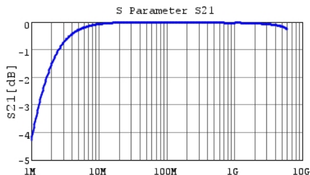
GRM1553U1A122JA01 S21 DCOV, 20degC
