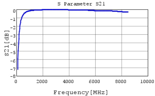
GRM1555C2A7R7CA01 S21 DC0V, 25degC
