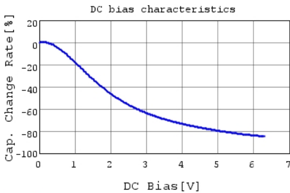
GRM155R60J106ME47 C-DC bias capchange, 25.0C
