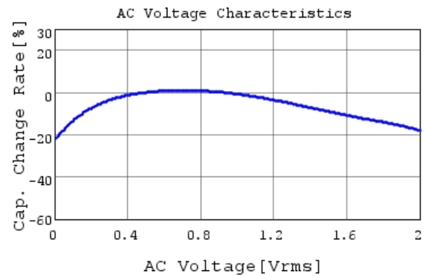
GRM155R60J106ME47 C-AC Voltage capchange, D
