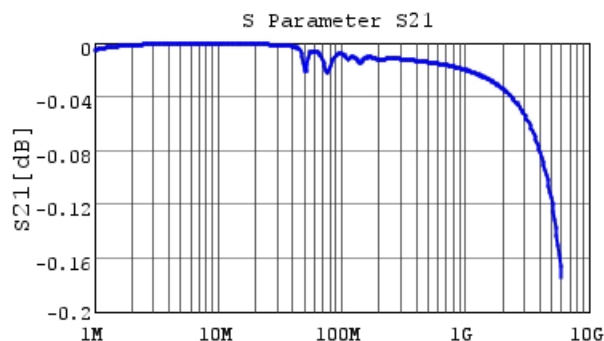
GRM31M5C2A473JA01 S21 DCOV, 25degC
