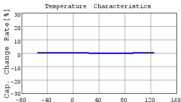
GRM31M5C2A473JA01 C-Temp. capchange, DCOV, 1
