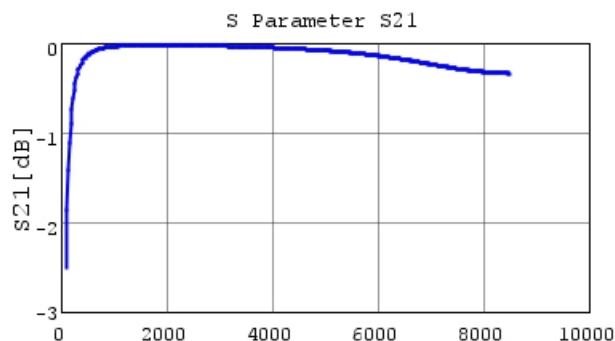
Frequency [MHz] GRT0335C1E180FA02 S21 DCOV, 25degC
