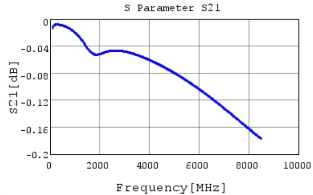
GRT0335C1E391JA02 S21 DCOV, 25degC
