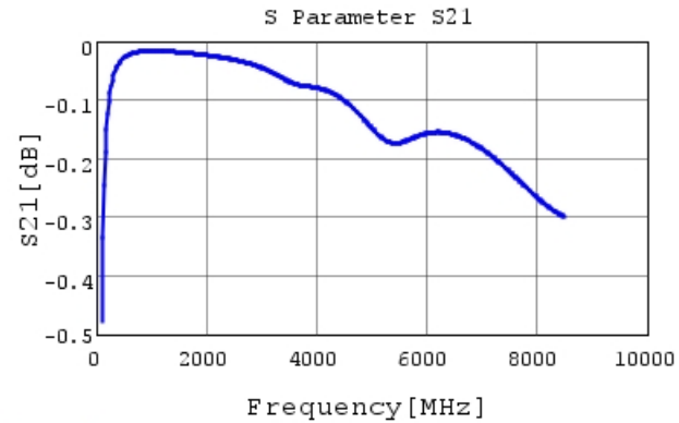
GRT0335C2A470JA02 S21 DCOV, 25degC
