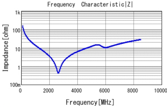
■ GRT1555C1H100JA02 |Z| DC0V, 25degC
