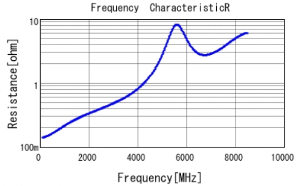
■ GRT1555C1H100JA02 R DC0V, 25degC
