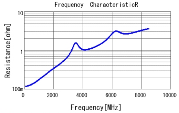
■ GRT1555C2A270JA02 R DC0V, 25degC
