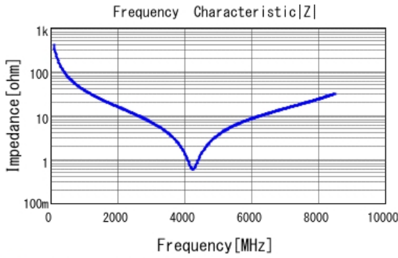
■ GRT1555C2A4R0CA02 |Z| DCOV, 25degC
