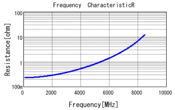
■ GRT1555C2A4R0CA02 R DCOV, 25degC
