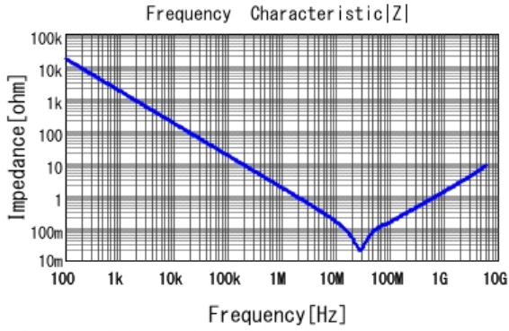
■ GRT155R71E104KE01 |Z| DC0V, 25degC
