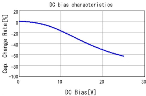
■ GRT155R71E104KE01 C-DC bias capchange, 25.0degC, AC1.
