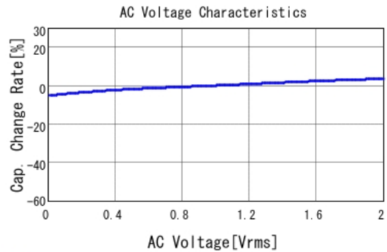
■ GRT155R71E104KE01 C-AC Voltage capchange, DC0V, 25.0d
