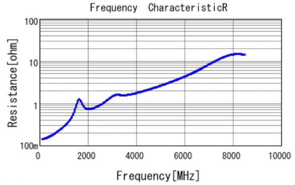
■ GRT1885C1H820JA02 R DCOV, 25degC
