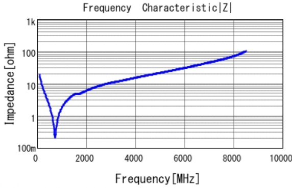
■ GRT1885C1H820JA02 |Z| DCOV, 25degC
