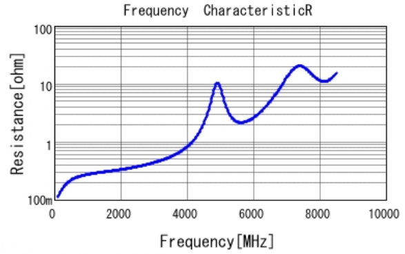
■ GRT1885C1H9R0DA02 R DCOV, 25degC
