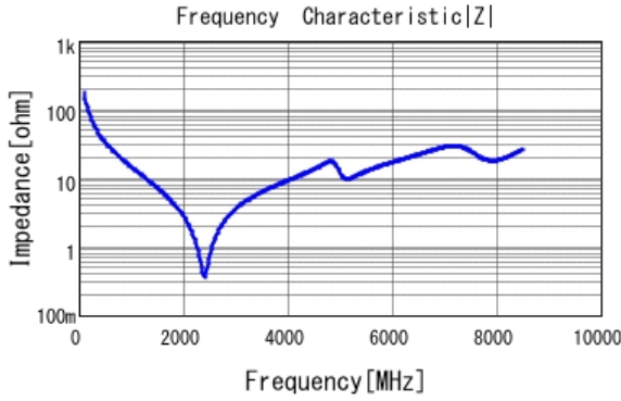
■ GRT1885C1H9R0DA02 |Z| DCOV, 25degC
