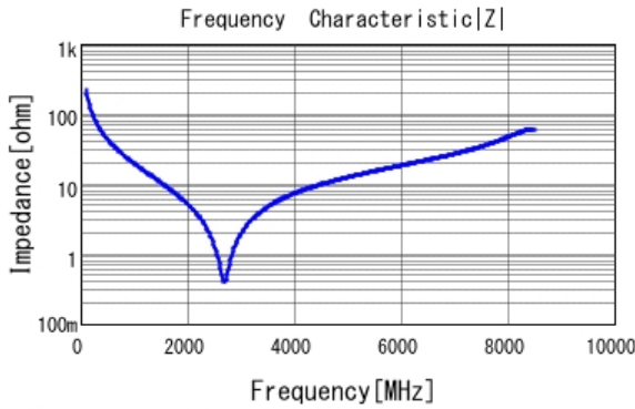
■ GRT1885C2A7R0DA02 |Z| DCOV, 25degC
