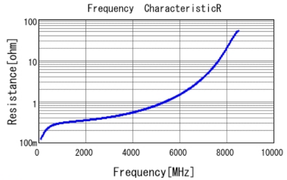
■ GRT1885C2A7R0DA02 R DCOV, 25degC
