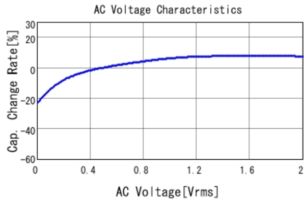
■ NFM15HC105D0G3 C-AC Voltage capchange, DCOV, 25.0c
