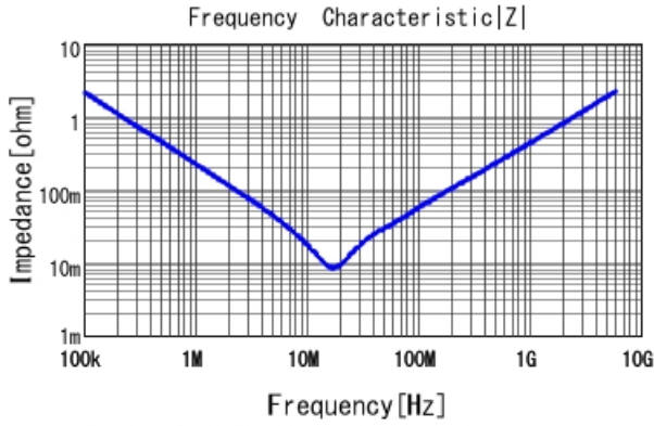
■ NFM15HC105D0G3 |Z| DCOV, 25degC, Non-feedthrough
