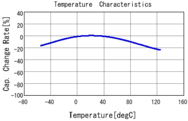
■ NFM15HC105D0G3 C-Temp. capchange, DCOV, ACO. 15Vrms
