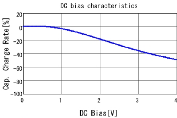
■ NFM15HC105D0G3 C-DC bias capchange, 25.0degC, AC0.
