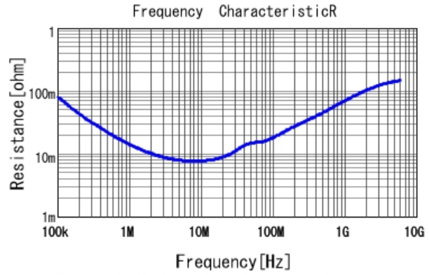
■ NFM15HC105D0G3 R DCOV, 25degC, Non-feedthrough
