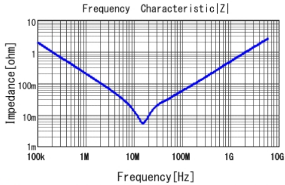
■ NFM18HC105C1C3 |Z| DC0V, 25degC, Non-feedthrough
