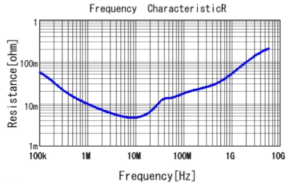
■ NFM18HC105C1C3 R DC0V, 25degC, Non-feedthrough
