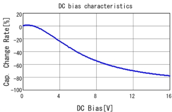
■ NFM18HC105C1C3 C-DC bias capchange, 25.0degC, AC1Vrms
