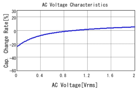
■ NFM18HC105C1C3 C-AC Voltage capchange, DC0V, 25.0degC
