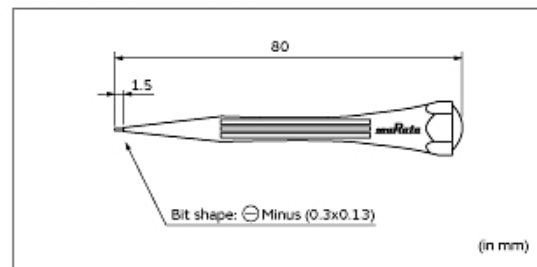
Recommended Screwdriver
