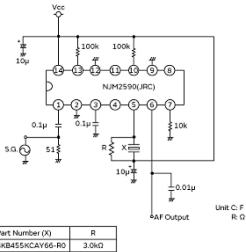
Measurement Circuit
