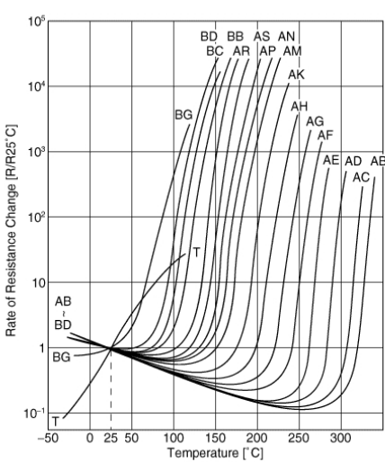
Resistance-Temperature Charac.
