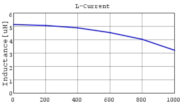
1225AS-H-4R7M L-Current 20degC
