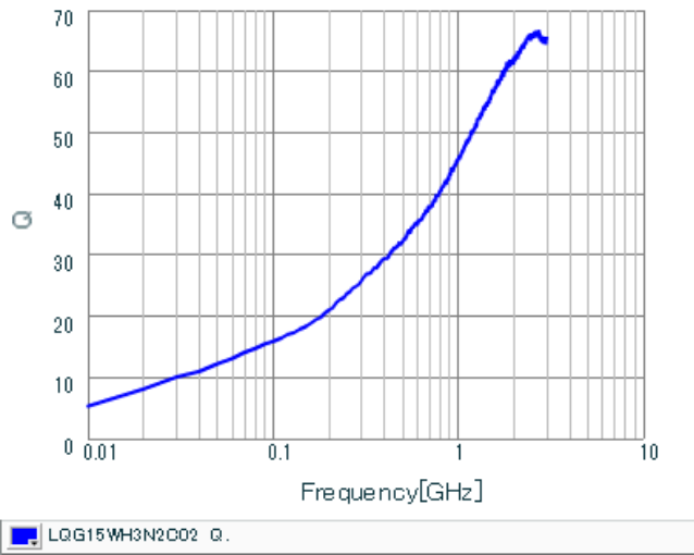
Q-Frequency Characteristics
