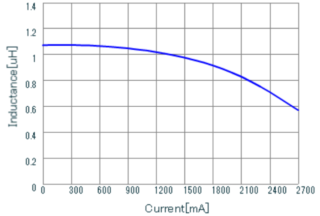
LQH2HPN1R0NJR DC-Bias, 20
