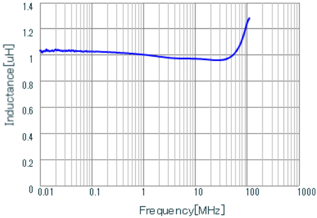
LQH2HPN1R0NJR L
