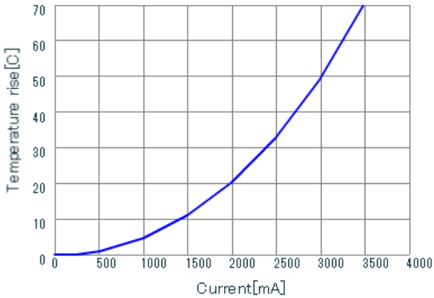
LQH2HPN1R0NJR DT_Current
