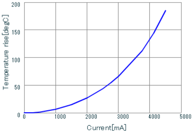
LQH3NPN2R2MME DT_Current
