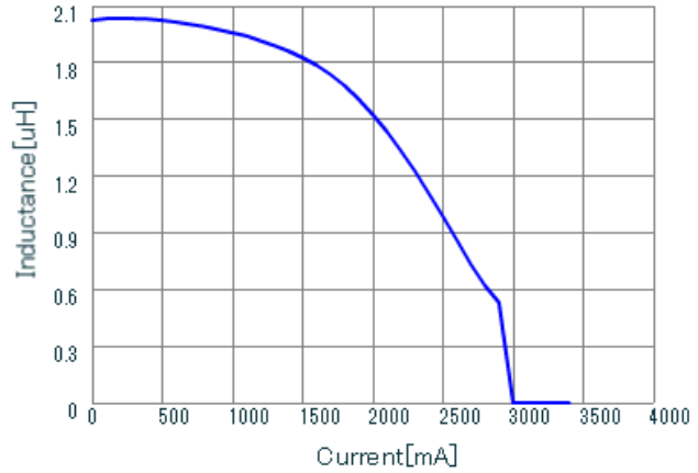
LQH3NPN2R2MME DC-Bias, 20
