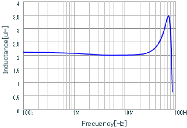
LQH3NPN2R2MME L
