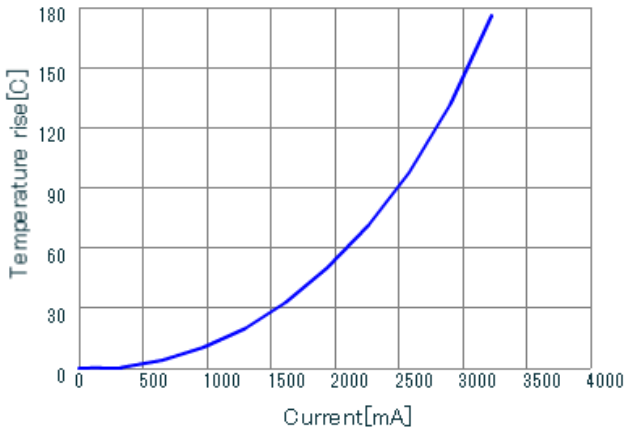
LQH3NPN3R3MGR DT_Current
