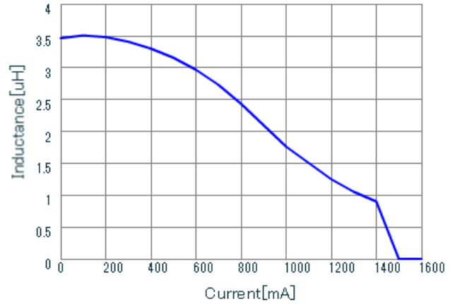
LQH3NPN3R3MGR DC-Bias, 20
