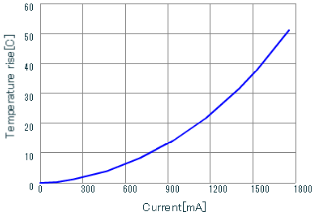
LQH43PB100M26 DT_Current
