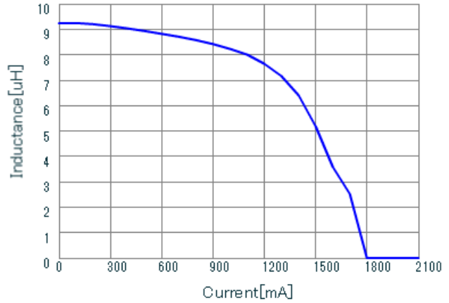
LQH43PB100M26 DC-Bias, 20
