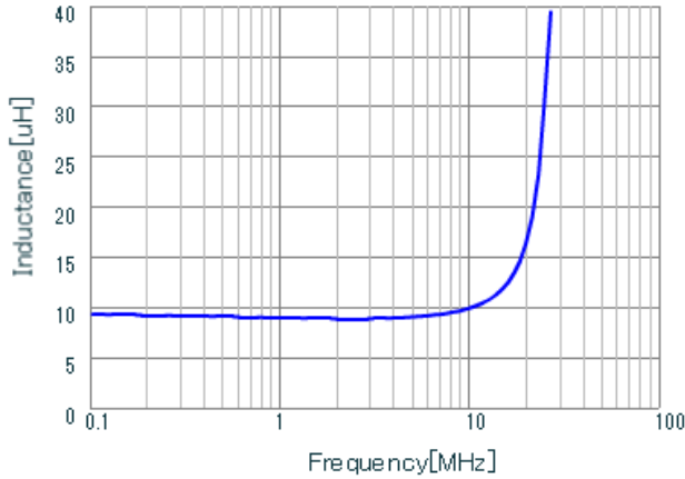
LQH43PB100M26 L
