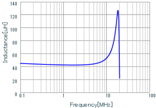
LQH44PN470MJ0 L
