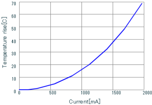
LQH44PN6R8MGR DT_Current
