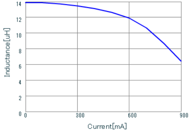
LQH44PZ150MGR DC-Bias, 20
