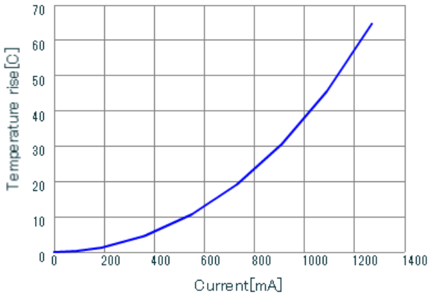
LQH44PZ150MGR DT_Current
