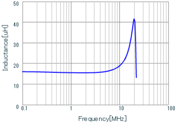
LQH44PZ150MGR L
