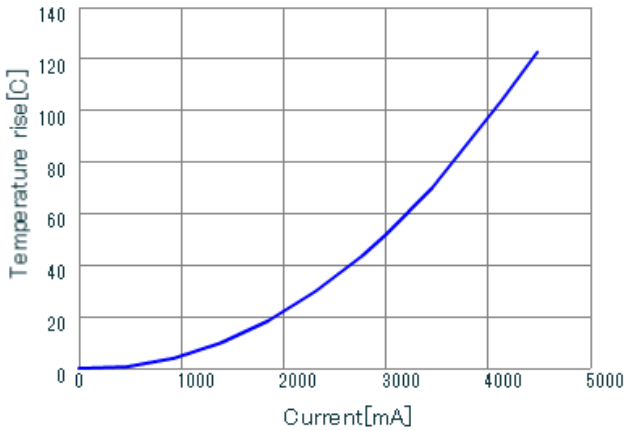
LQH5BPN3R3NT0 DT_Current
