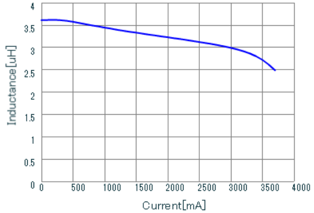
LQH5BPN3R3NT0 DC-Bias, 20
