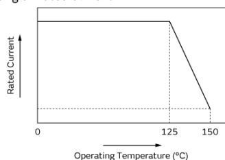
Derating of Rated Current
